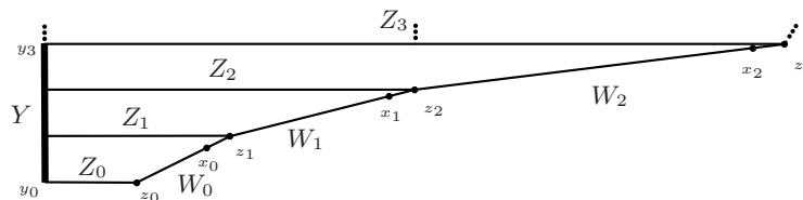
Figure 3: (\rho_1, 2) -contraction
